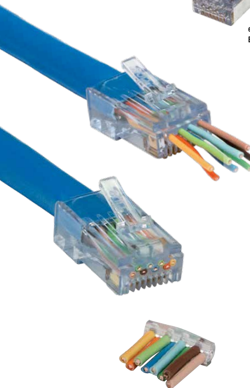
Wires protrude from the front of the connector before being trimmed flush.
