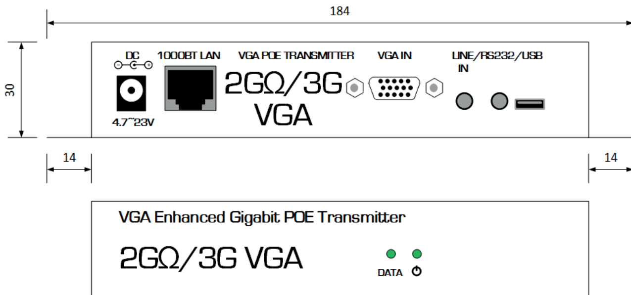
716VGA Front/Back
